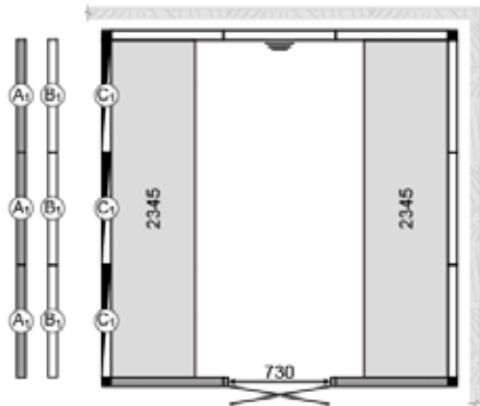
PANACEA STEAM 2525 Size 2525 x 2525 mm Item no. 9607 5084 With door opening 930 mm Item no. 9607 5086
