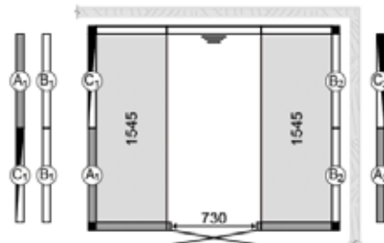
PANACEA STEAM 2117 Size 2125 x 1725 mm Item no. 9607 5076
