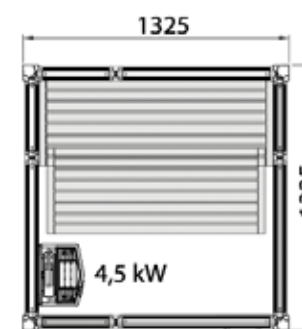
IMPRESSION SAUNA i1313 White: Item no. 9607 4820 Black: Item no. 9607 4822
