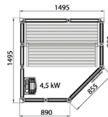
IMPRESSION SAUNA i1515/C White: Item no. 9607 4805 Black: Item no. 9607 4807
