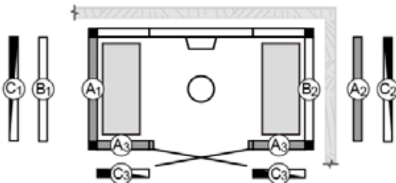
PANACEA 1709 TX WITH STEAM COLUMN AND CEILING SHOWER Size 1725 x 925 mm Item no. 9607 5034
