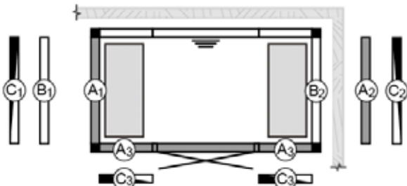
PANACEA STEAM 1709 T WITH STEAM OUTLET Size 1725 x 925 mm Item no. 9607 5022. Accompany with steam generator.
