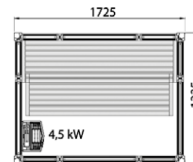
IMPRESSION SAUNA i1713 White: Item no. 9607 4825 Black: Item no. 9607 4827
