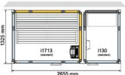
TWIN 130/1713/W White Item no. 9607 4856 Black Item no. 9607 4857
