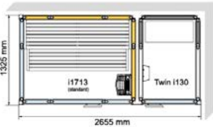
TWIN 130/1713 White Item no. 9607 4844 Black Item no. 9607 4845
