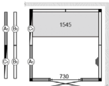
PANACEA STEAM 1717 Size 1725 x 1725 mm Item no. 9607 5070 With door opening 930 mm Item no. 9607 5072
