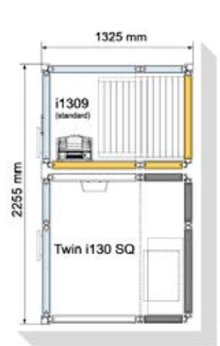
TWIN 130 SQ/1309 White Item no. 9607 4846 Black Item no. 9607 4847
