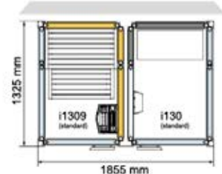
TWIN 130/1309/W White Item no. 9607 4852 Black Item no. 9607 4853
