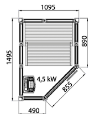
IMPRESSION SAUNA i1115/C White: Item no. 9607 4800 Black: Item no. 9607 4802
