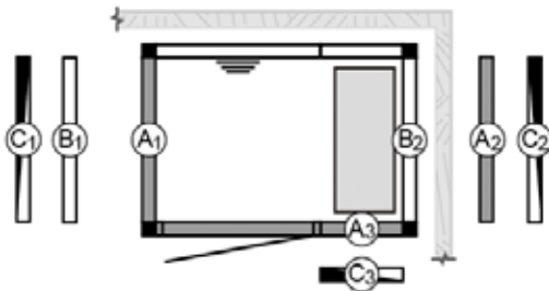
PANACEA STEAM 1309 WITH STEAM OUTLET Size 1325 x 925 mm Item no. 9607 5020. Accompany with steam generator.
