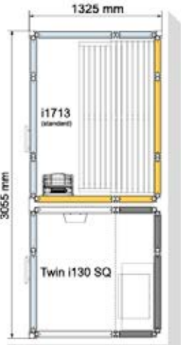
TWIN 130 SQ/1713 White Item no. 9607 4850 Black Item no. 9607 4851
