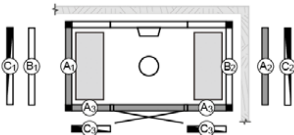
PANACEA 1709 TX/T WITH STEAM COLUMN AND CEILING SHOWER Size 1725 x 925 mm Item no. 9607 5030
